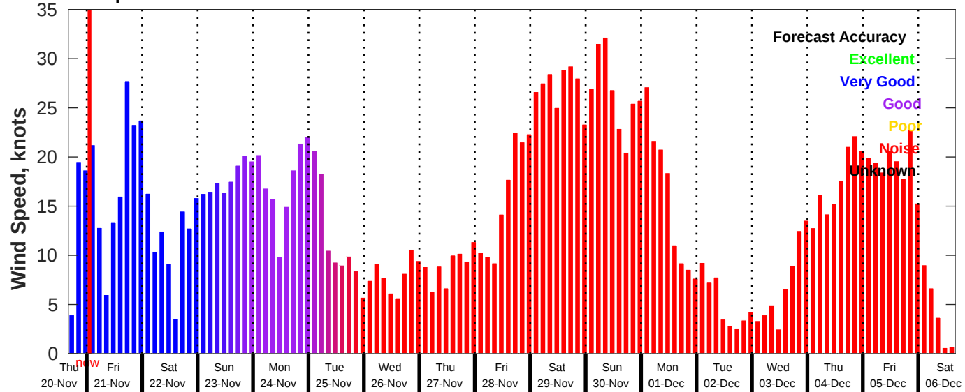
GFS Wind Speed Forecast for NDBC 46069 from 20-Nov-2025 16:00:00 to 06-Dec-2025 16:00:00
