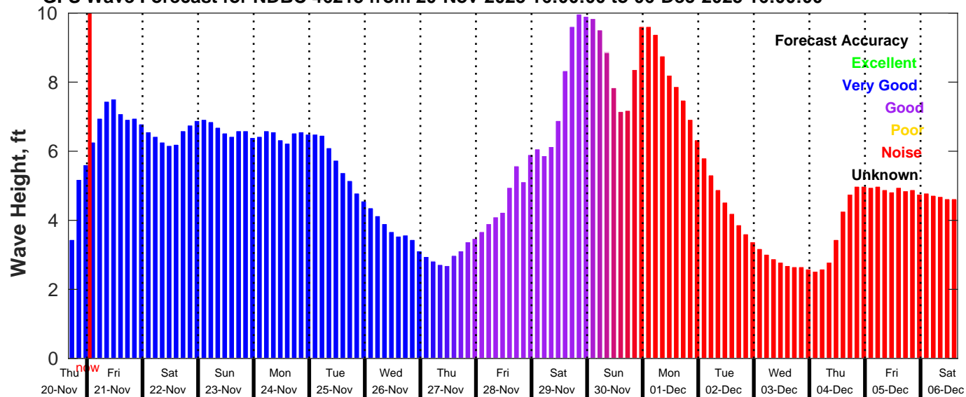
GFS Wave Forecast for NDBC 46215 from 20-Nov-2025 16:00:00 to 06-Dec-2025 16:00:00
