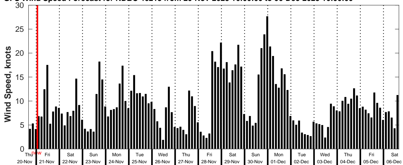
GFS Wind Speed Forecast for NDBC 46215 from 20-Nov-2025 16:00:00 to 06-Dec-2025 16:00:00
