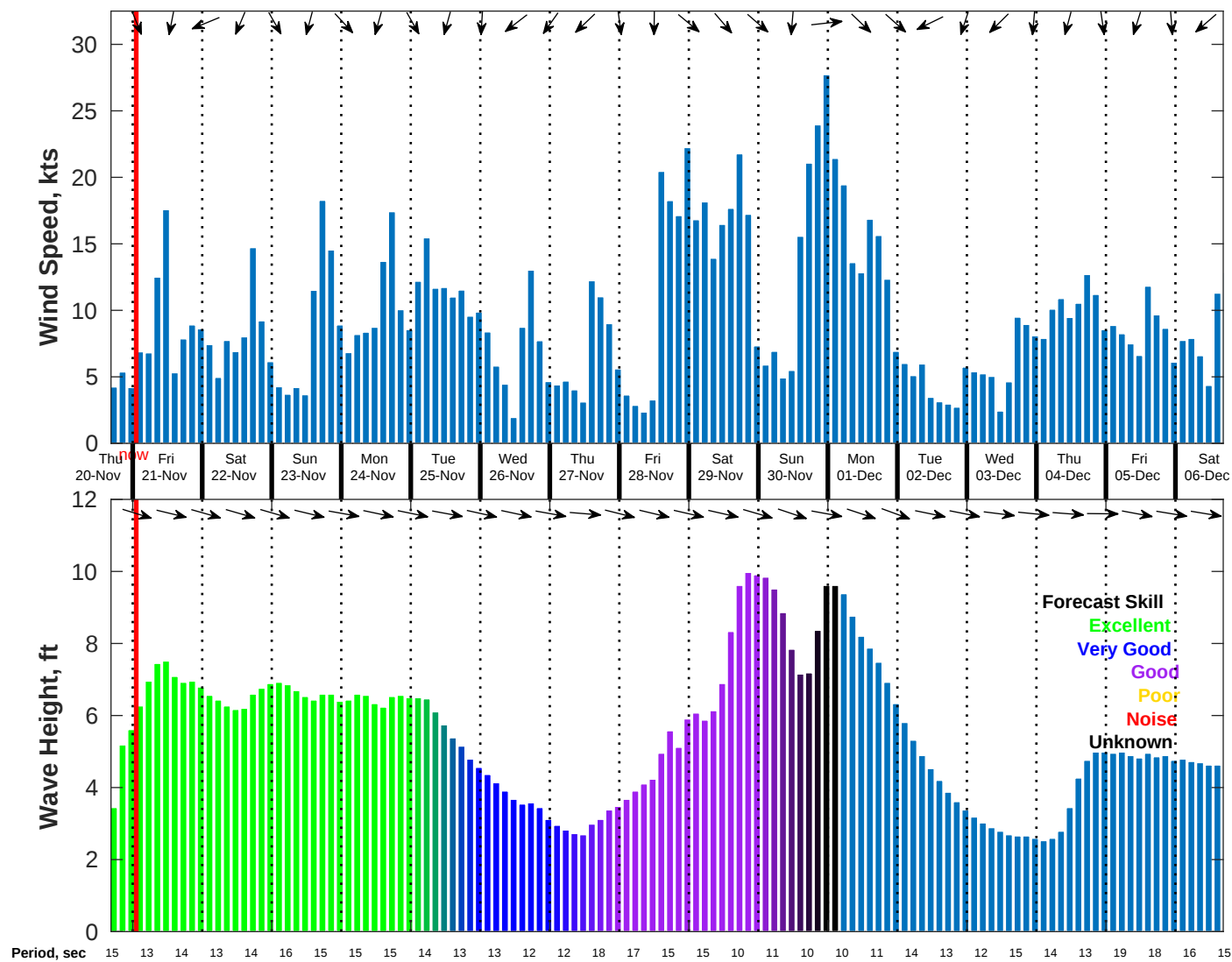
Wind & Wave Forecast for NDBC 46215 from 20-Nov-2025 16:00:00 to 06-Dec-2025 16:00:00
