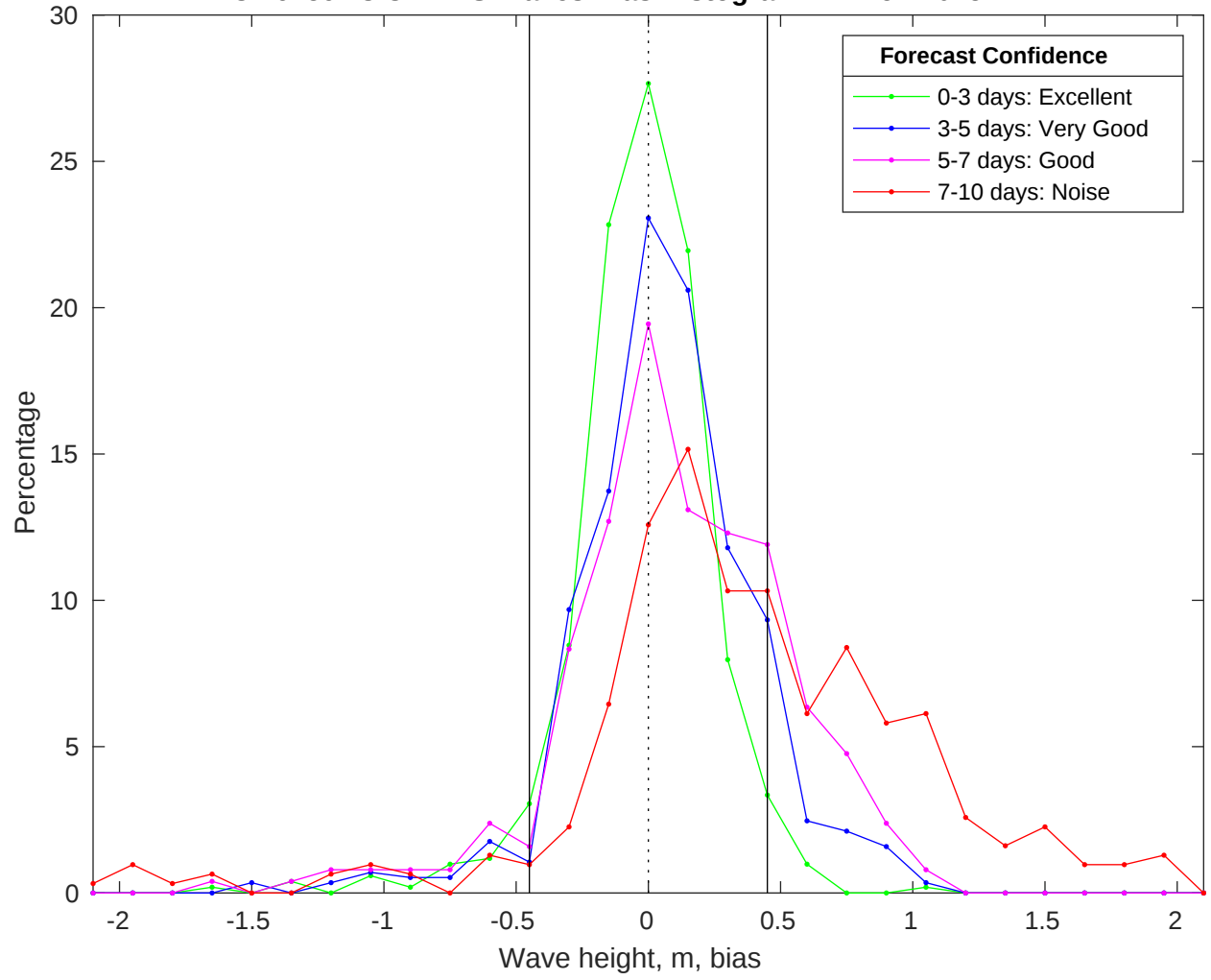
NDBC 46259 vs CMEMS Waves Bias Histogram: 21-Nov-2025
