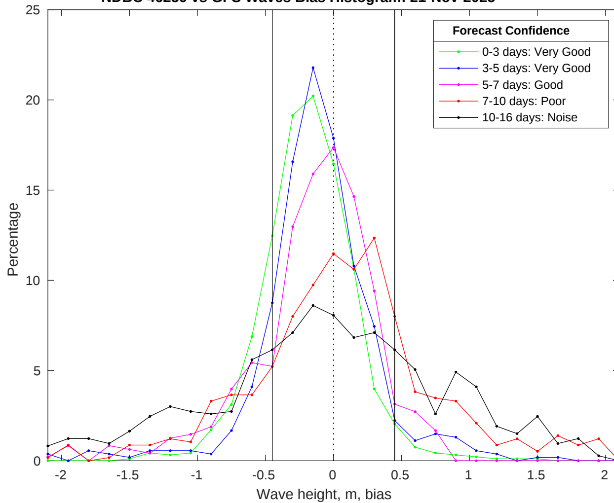
NDBC 46259 vs GFS Waves Bias Histogram: 21-Nov-2025
