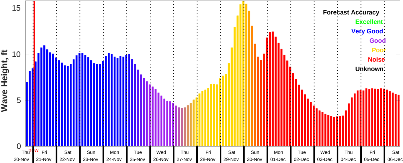
GFS Wave Forecast for NDBC 46259 from 20-Nov-2025 16:00:00 to 06-Dec-2025 16:00:00
