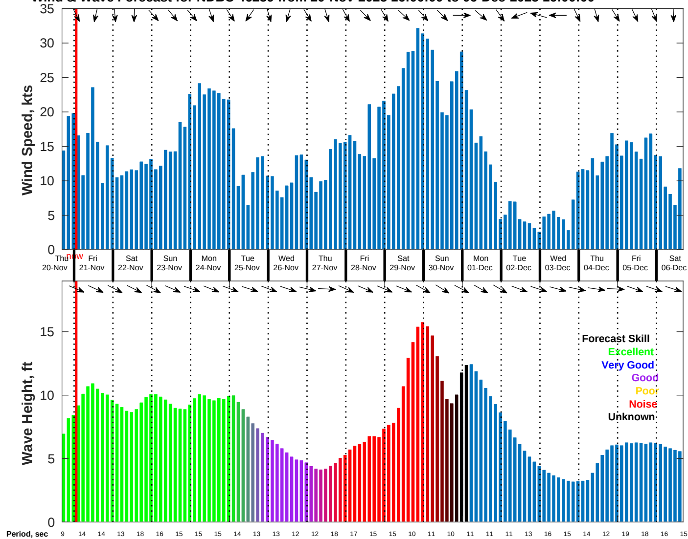
Wind & Wave Forecast for NDBC 46259 from 20-Nov-2025 16:00:00 to 06-Dec-2025 16:00:00
