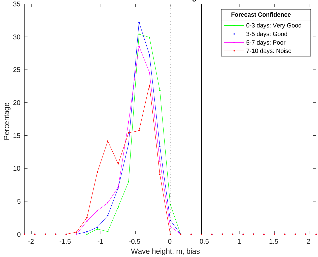
NDBC 51209 vs CMEMS Waves Bias Histogram: 21-Nov-2025
