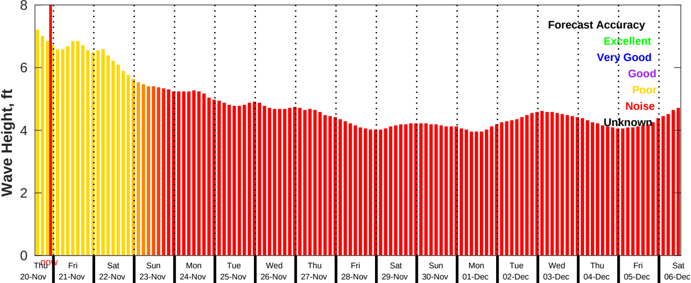
GFS Wave Forecast for NDBC 51209 from 20-Nov-2025 13:00:00 to 06-Dec-2025 13:00:00
