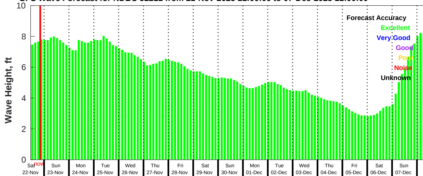
GFS Wave Forecast for NDBC 52211 from 21-Nov-2025 11:00:00 to 07-Dec-2025 11:00:00
