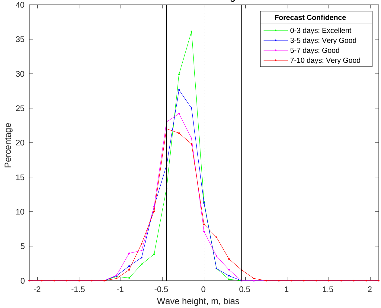
NDBC 52213 vs CMEMS Waves Bias Histogram: 21-Nov-2025
