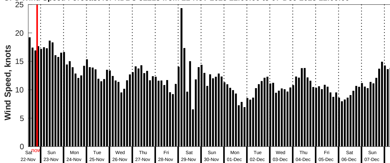
GFS Wind Speed Forecast for NDBC 52213 from 21-Nov-2025 11:00:00 to 07-Dec-2025 11:00:00
