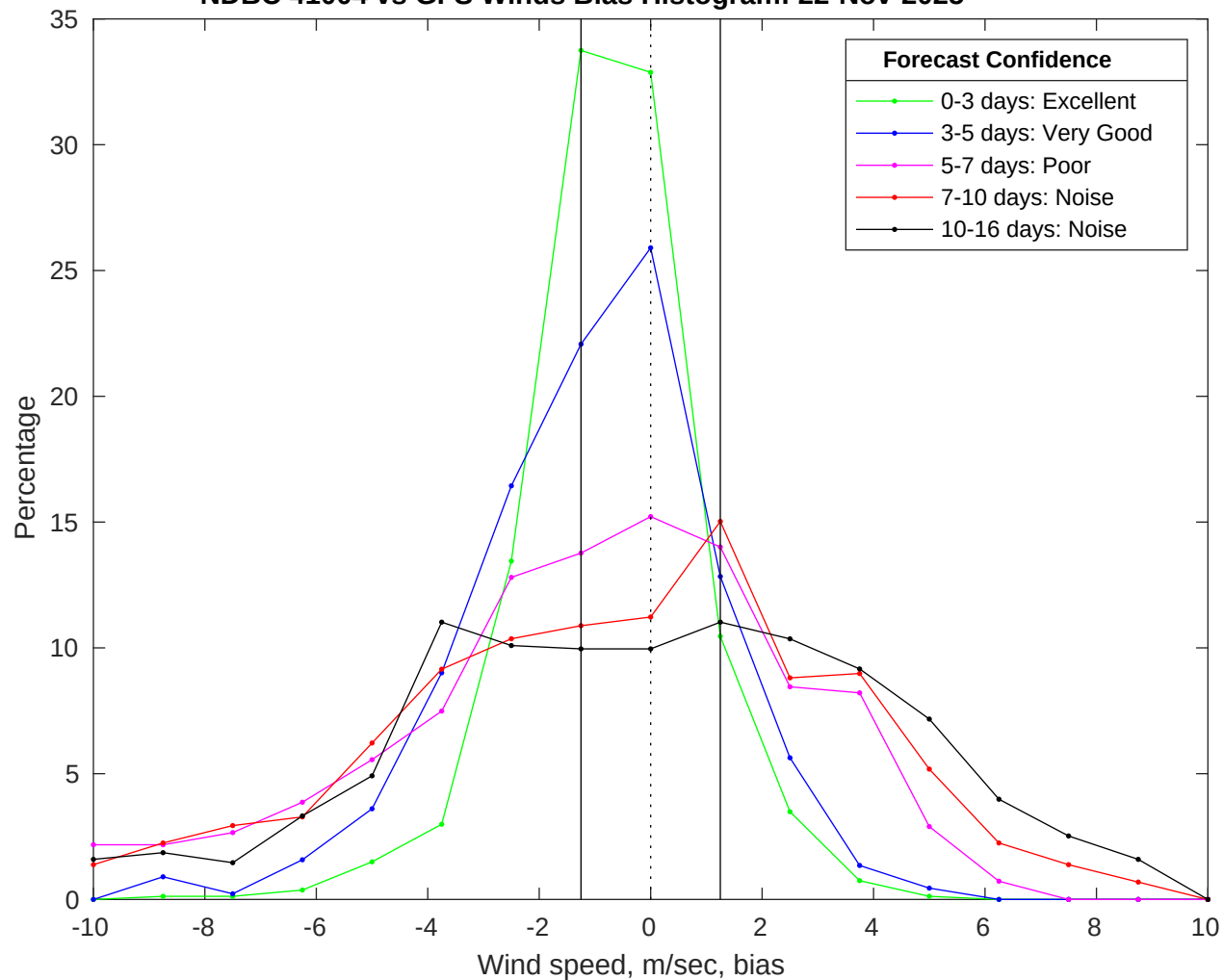
NDBC 41004 vs GFS Winds Bias Histogram: 22-Nov-2025
