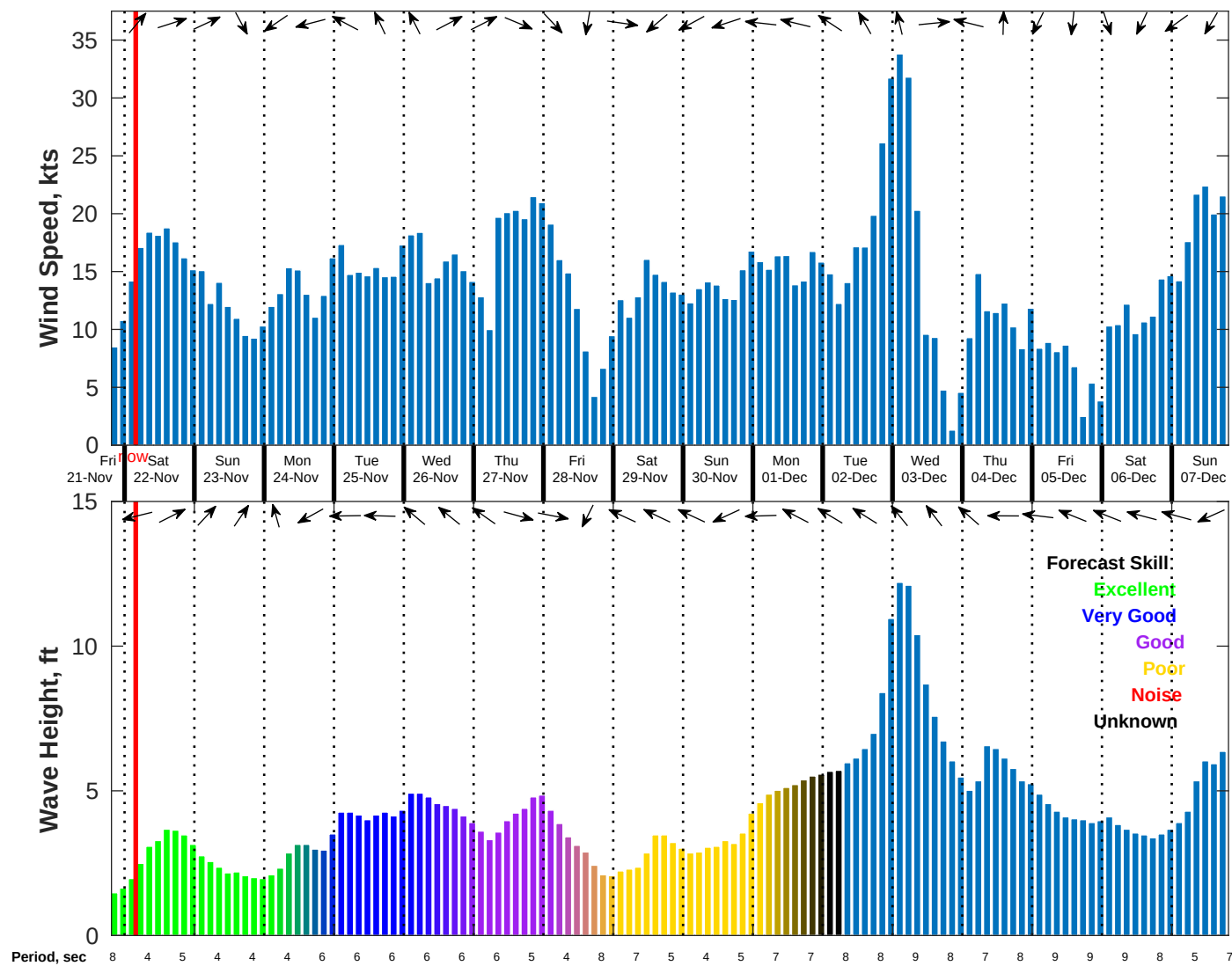
Wind & Wave Forecast for NDBC 41004 from 21-Nov-2025 19:00:00 to 07-Dec-2025 19:00:00
