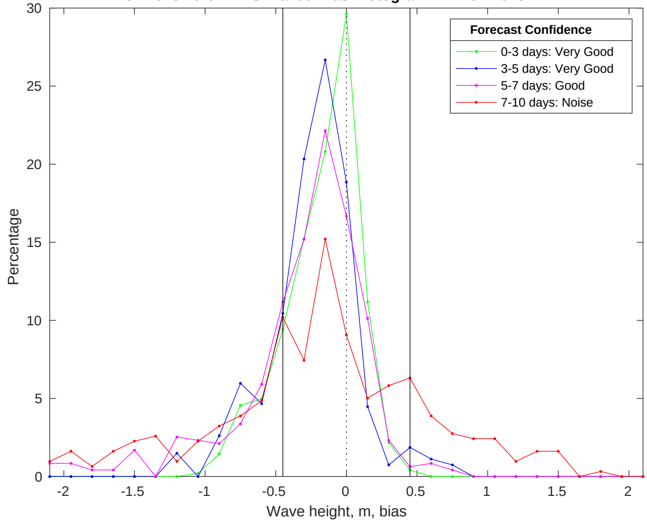
NDBC 41013 vs CMEMS Waves Bias Histogram: 22-Nov-2025
