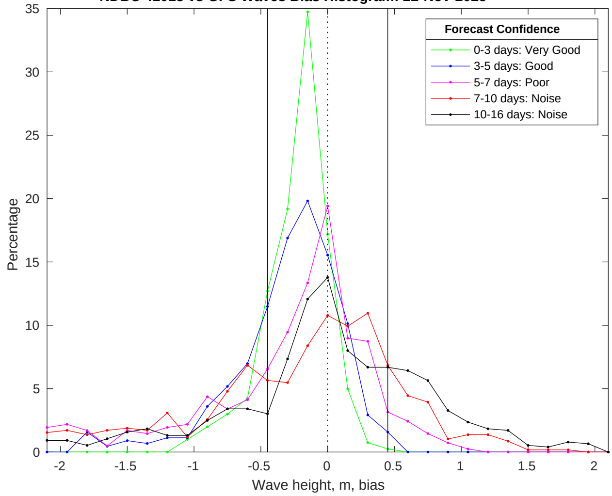
NDBC 41013 vs GFS Waves Bias Histogram: 22-Nov-2025
