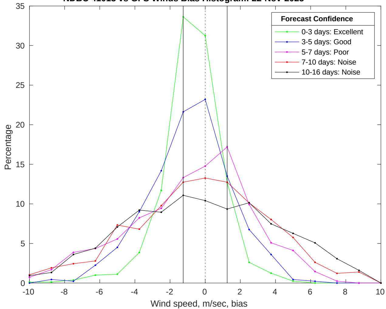
NDBC 41013 vs GFS Winds Bias Histogram: 22-Nov-2025
