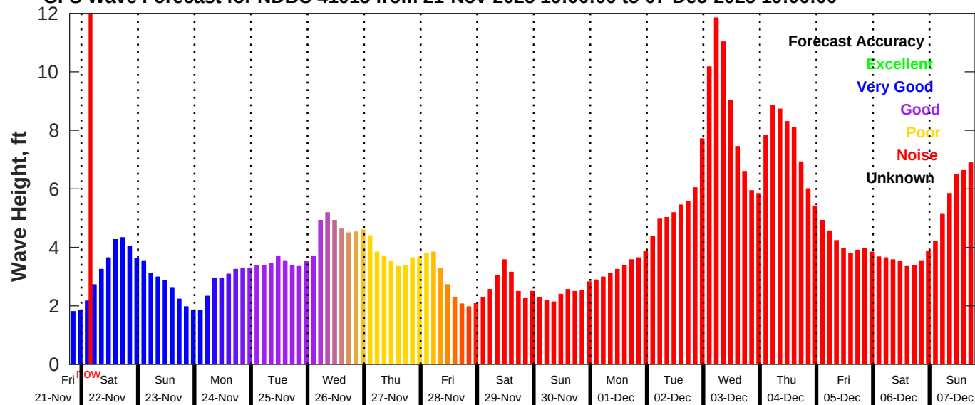
GFS Wave Forecast for NDBC 41013 from 21-Nov-2025 19:00:00 to 07-Dec-2025 19:00:00
