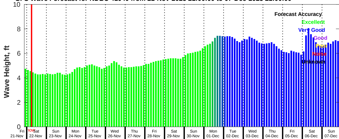
GFS Wave Forecast for NDBC 41040 from 21-Nov-2025 21:00:00 to 07-Dec-2025 21:00:00
