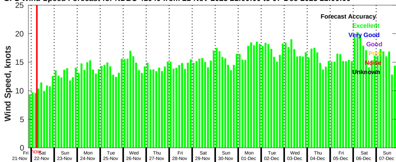
GFS Wind Speed Forecast for NDBC 41040 from 21-Nov-2025 21:00:00 to 07-Dec-2025 21:00:00
