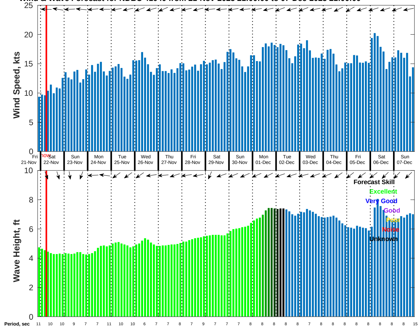
Wind & Wave Forecast for NDBC 41040 from 21-Nov-2025 21:00:00 to 07-Dec-2025 21:00:00
