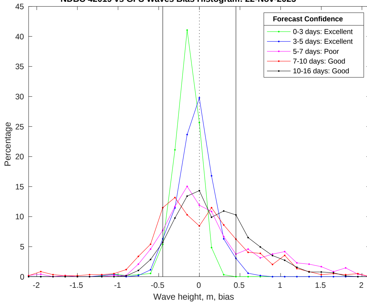
NDBC 42019 vs GFS Waves Bias Histogram: 22-Nov-2025
