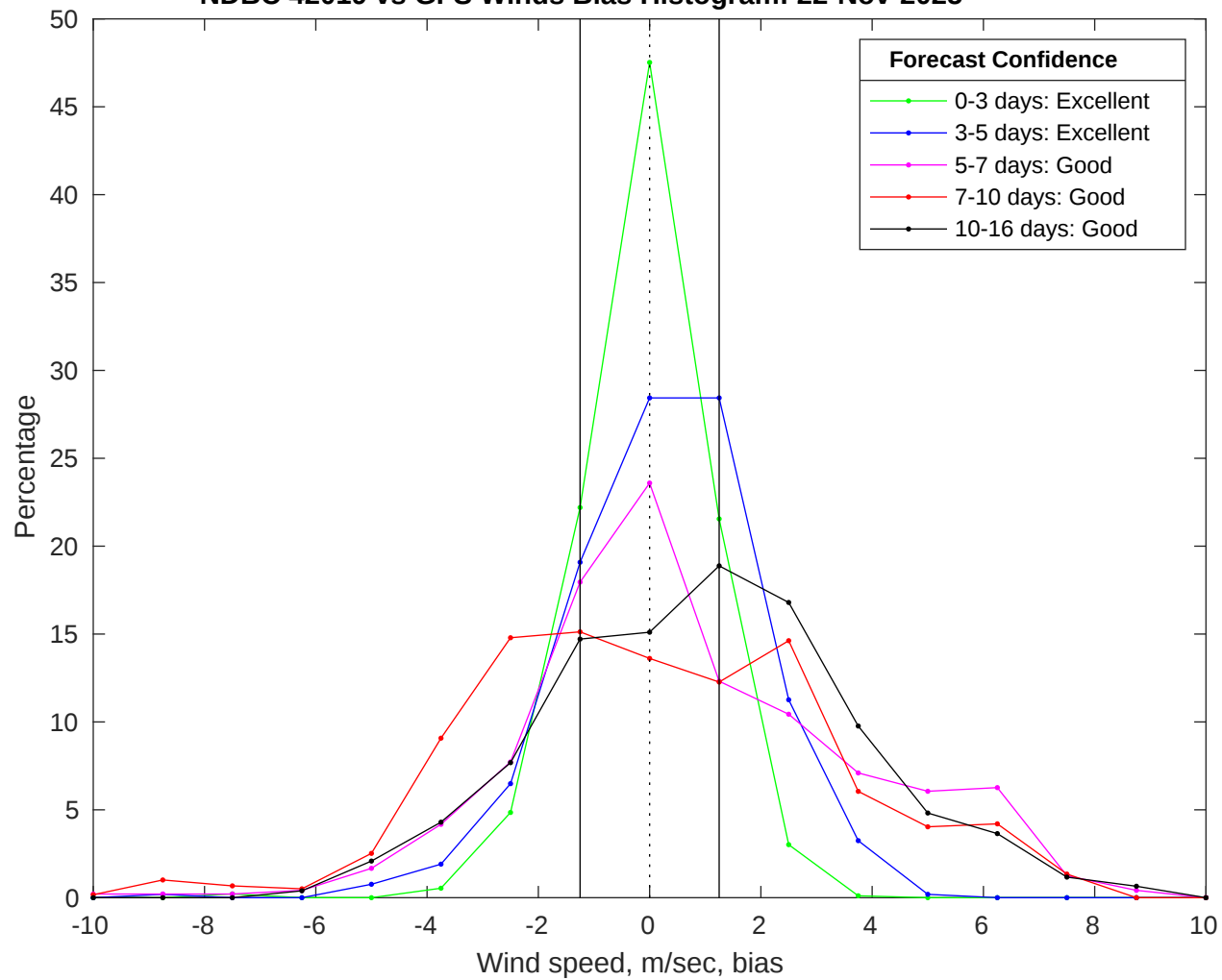
NDBC 42019 vs GFS Winds Bias Histogram: 22-Nov-2025
