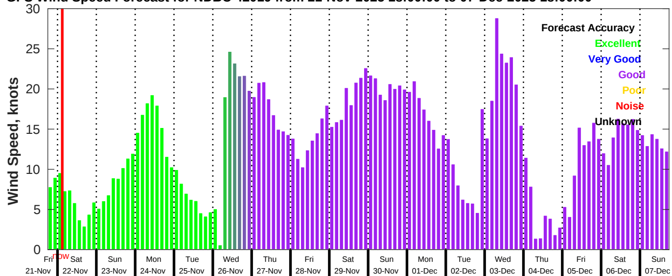
GFS Wind Speed Forecast for NDBC 42019 from 21-Nov-2025 18:00:00 to 07-Dec-2025 18:00:00
