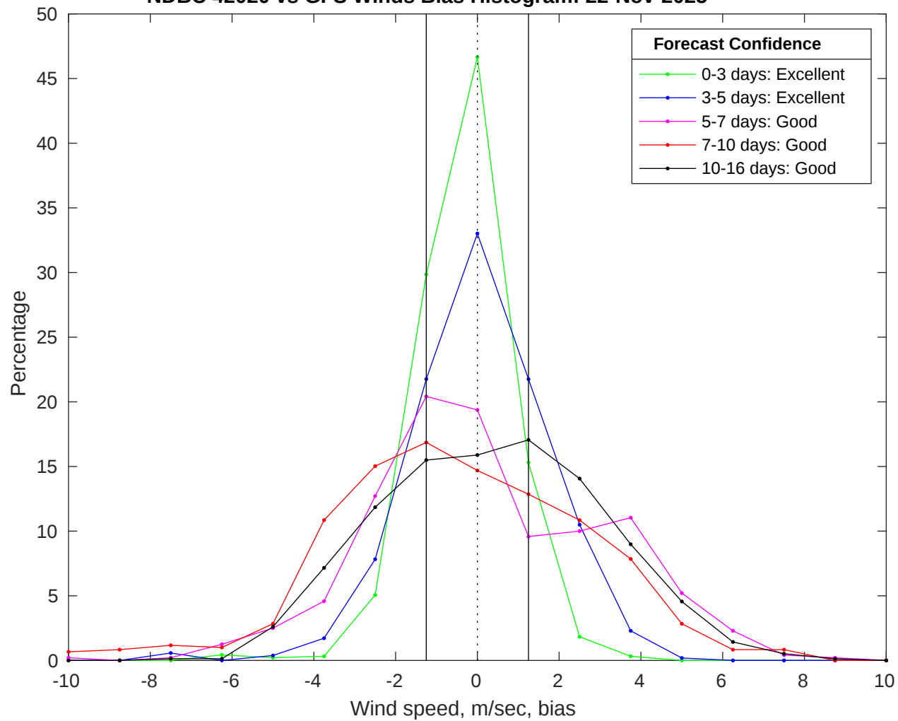
NDBC 42020 vs GFS Winds Bias Histogram: 22-Nov-2025
