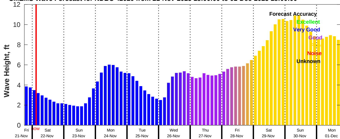
CMEMS Wave Forecast for NDBC 42020 from 21-Nov-2025 18:00:00 to 01-Dec-2025 18:00:00
