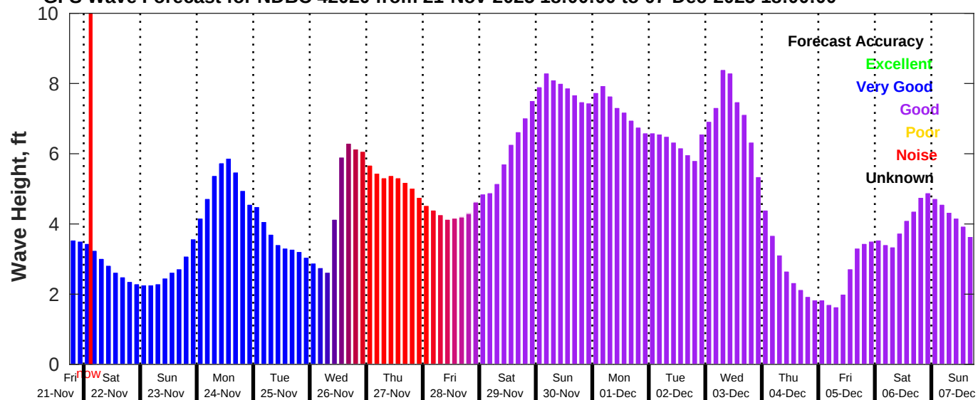
GFS Wave Forecast for NDBC 42020 from 21-Nov-2025 18:00:00 to 07-Dec-2025 18:00:00
