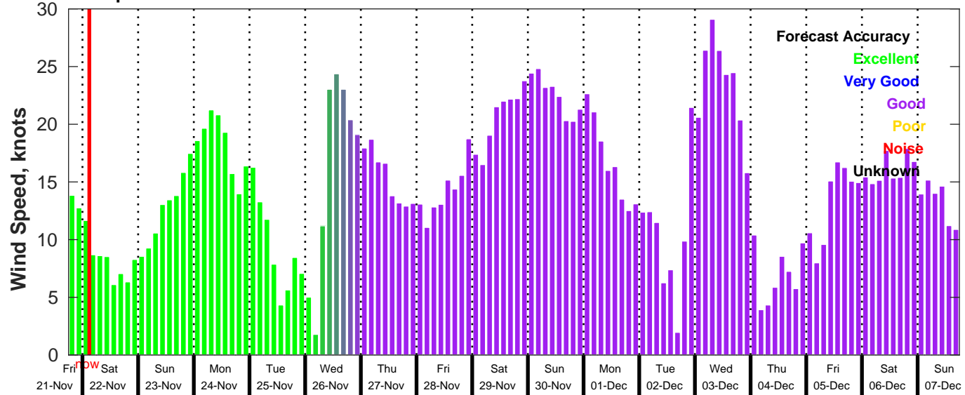
GFS Wind Speed Forecast for NDBC 42020 from 21-Nov-2025 18:00:00 to 07-Dec-2025 18:00:00
