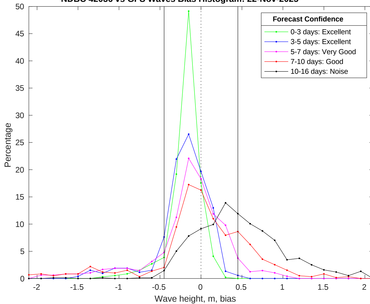
NDBC 42036 vs GFS Waves Bias Histogram: 22-Nov-2025
