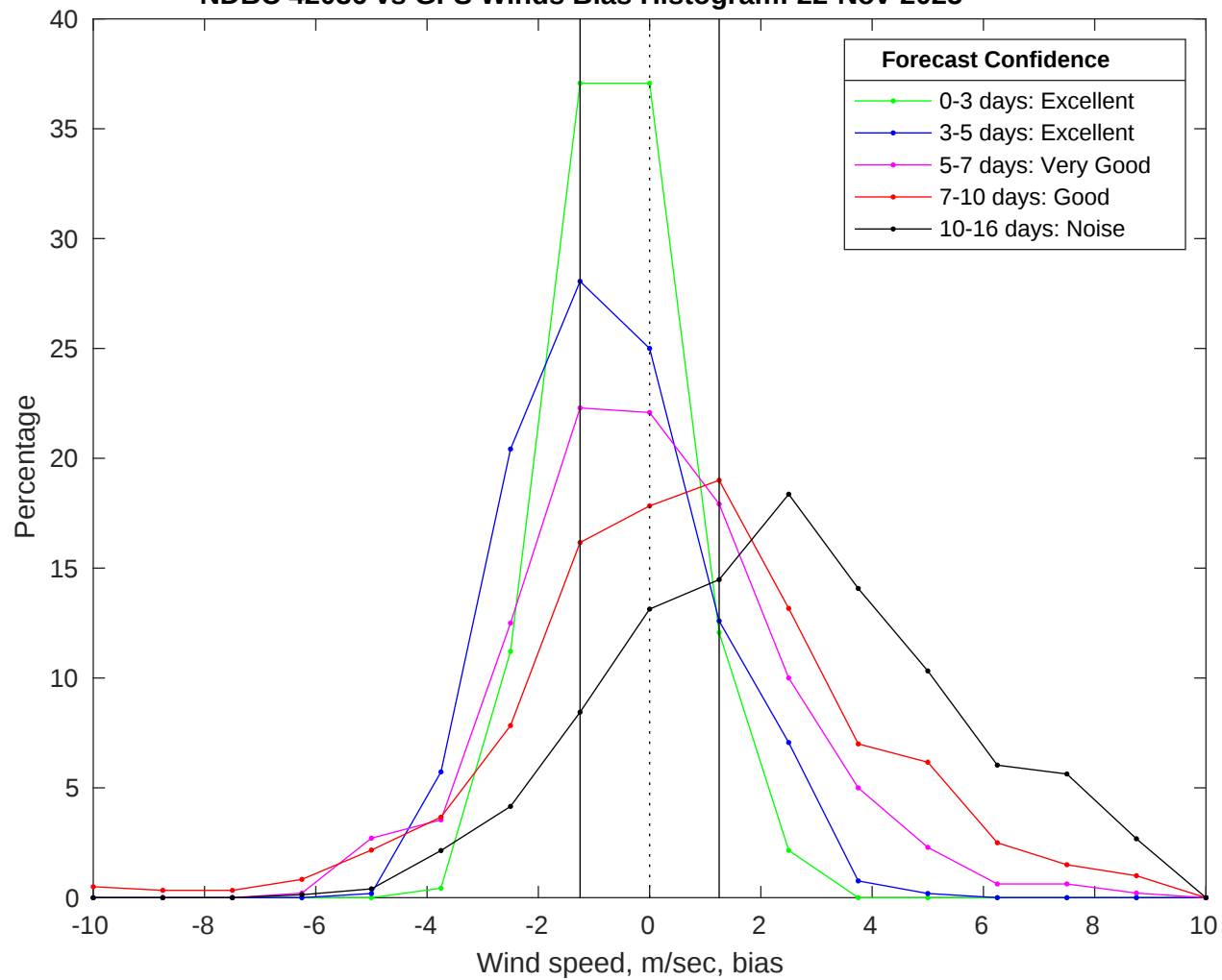
NDBC 42036 vs GFS Winds Bias Histogram: 22-Nov-2025
