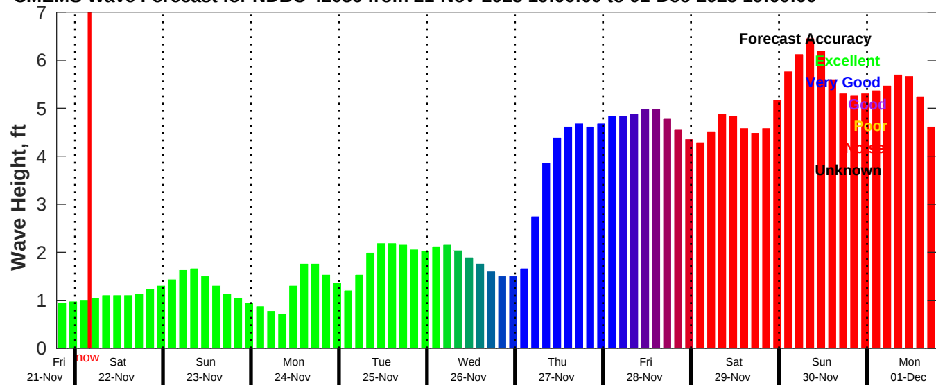
CMEMS Wave Forecast for NDBC 42036 from 21-Nov-2025 19:00:00 to 01-Dec-2025 19:00:00
