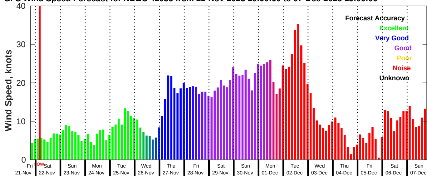
GFS Wind Speed Forecast for NDBC 42036 from 21-Nov-2025 19:00:00 to 07-Dec-2025 19:00:00
