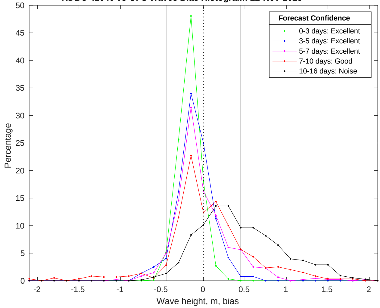
NDBC 42040 vs GFS Waves Bias Histogram: 22-Nov-2025
