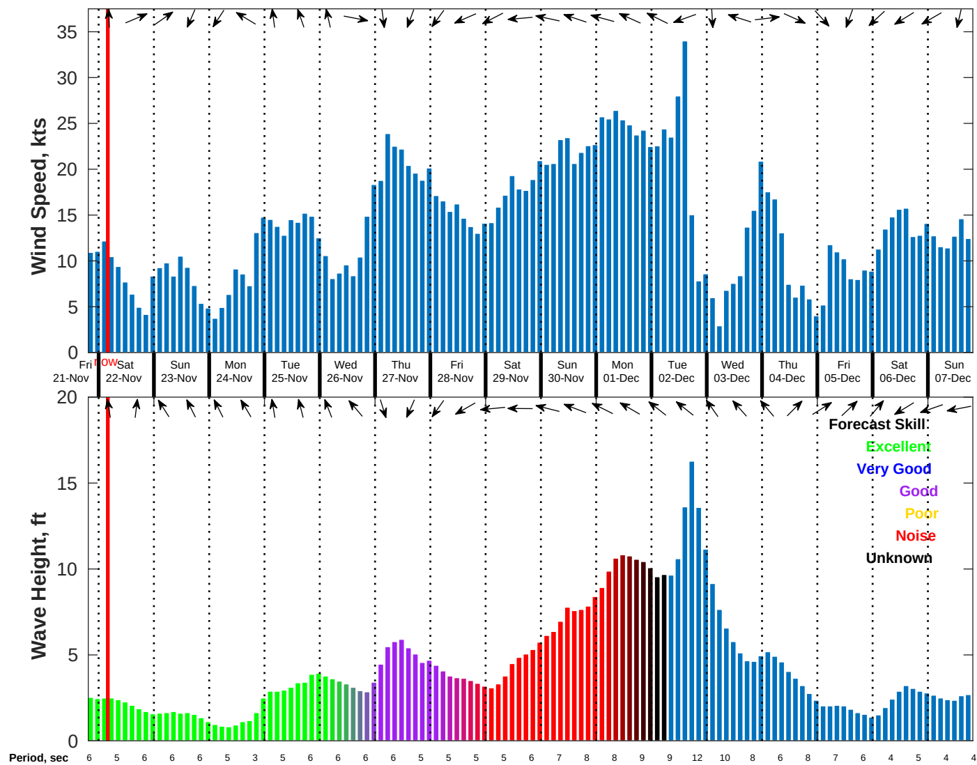
Wind & Wave Forecast for NDBC 42040 from 21-Nov-2025 19:00:00 to 07-Dec-2025 19:00:00
