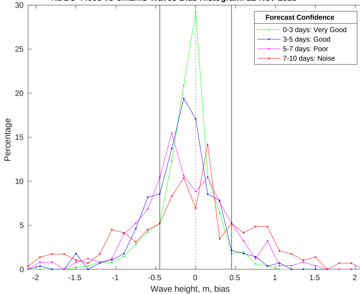
NDBC 44008 vs CMEMS Waves Bias Histogram: 22-Nov-2025
