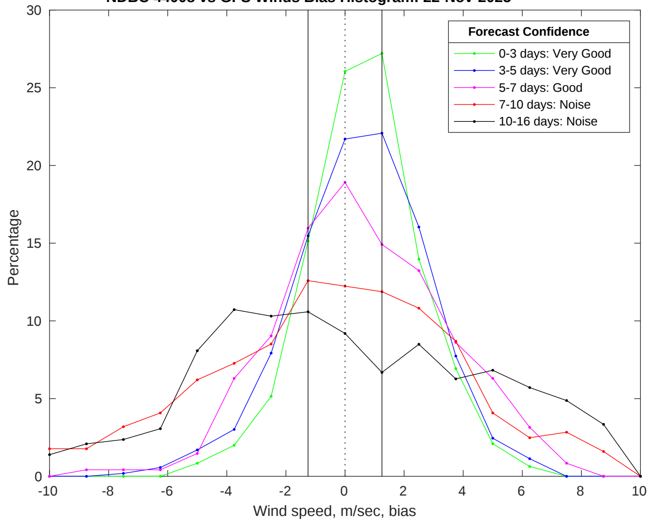
NDBC 44008 vs GFS Winds Bias Histogram: 22-Nov-2025
