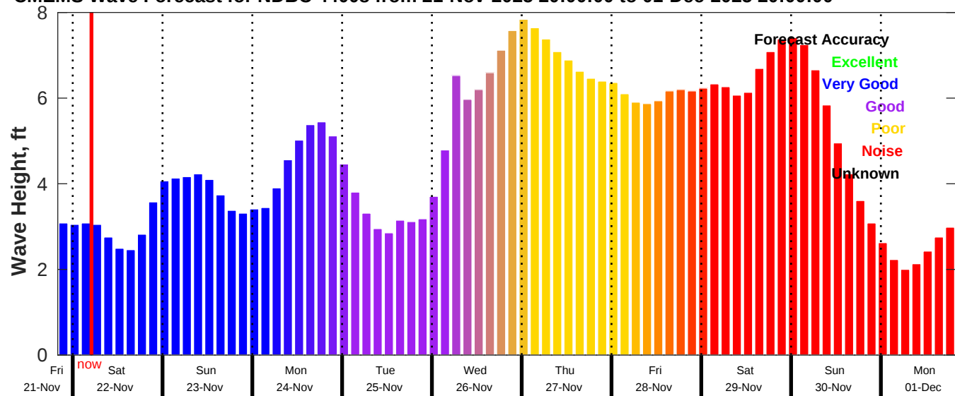
CMEMS Wave Forecast for NDBC 44008 from 21-Nov-2025 20:00:00 to 01-Dec-2025 20:00:00
