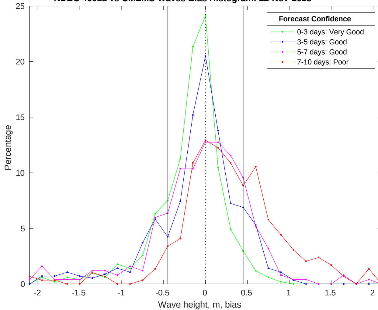
NDBC 46011 vs CMEMS Waves Bias Histogram: 22-Nov-2025
