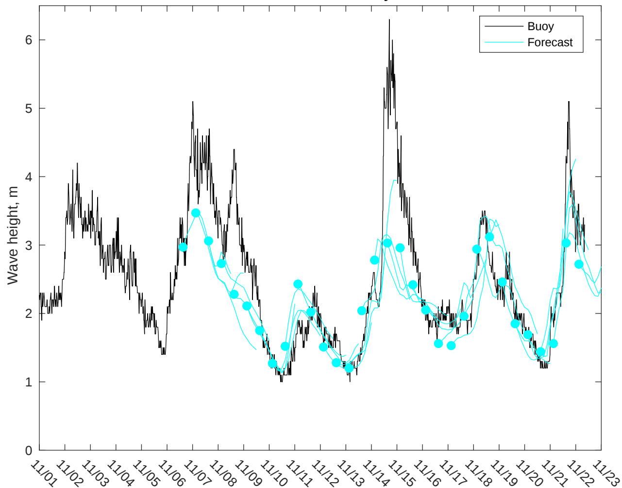
NDBC 46011 vs GFS Waves: 5 to 7 day forecast
