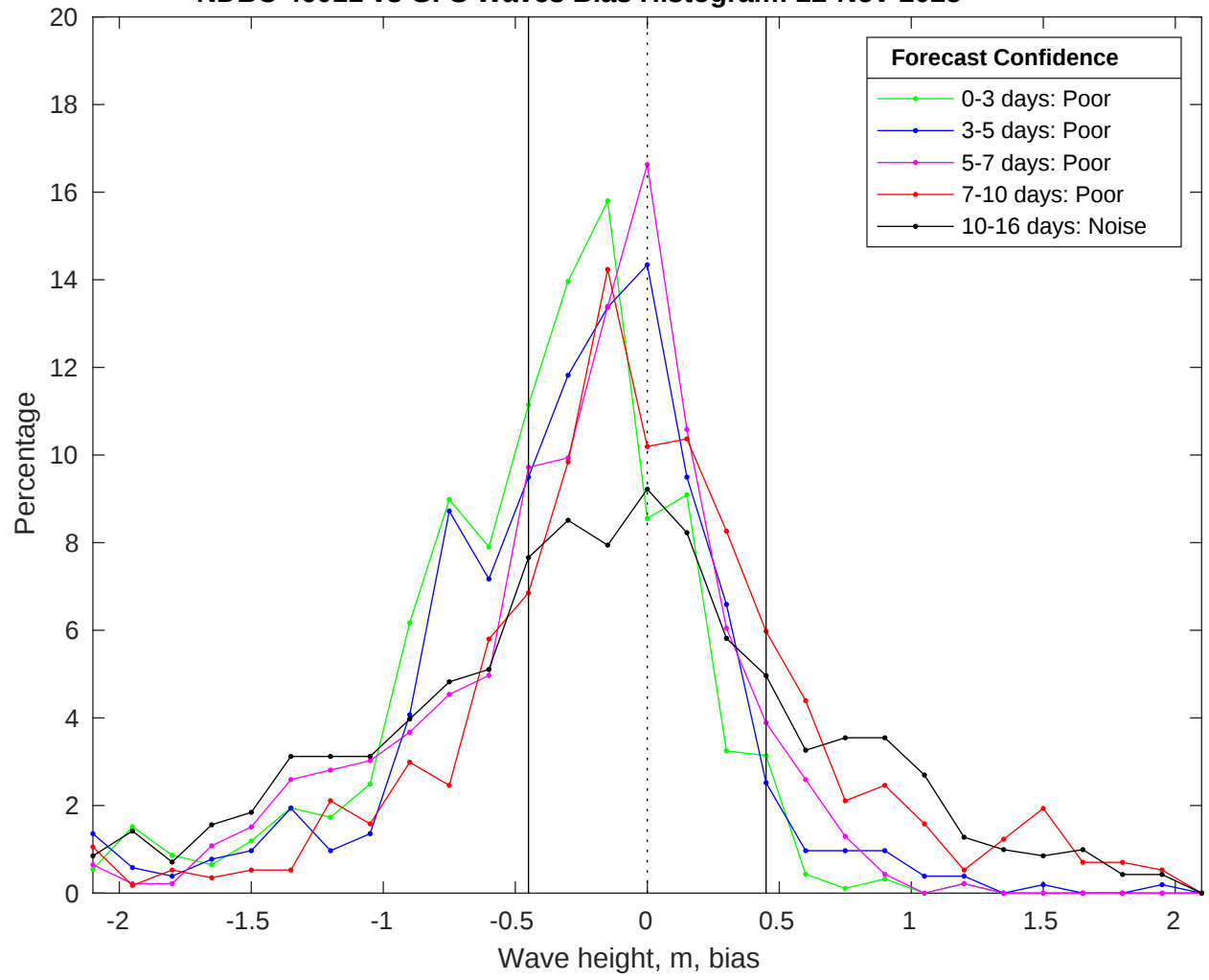
NDBC 46011 vs GFS Waves Bias Histogram: 22-Nov-2025
