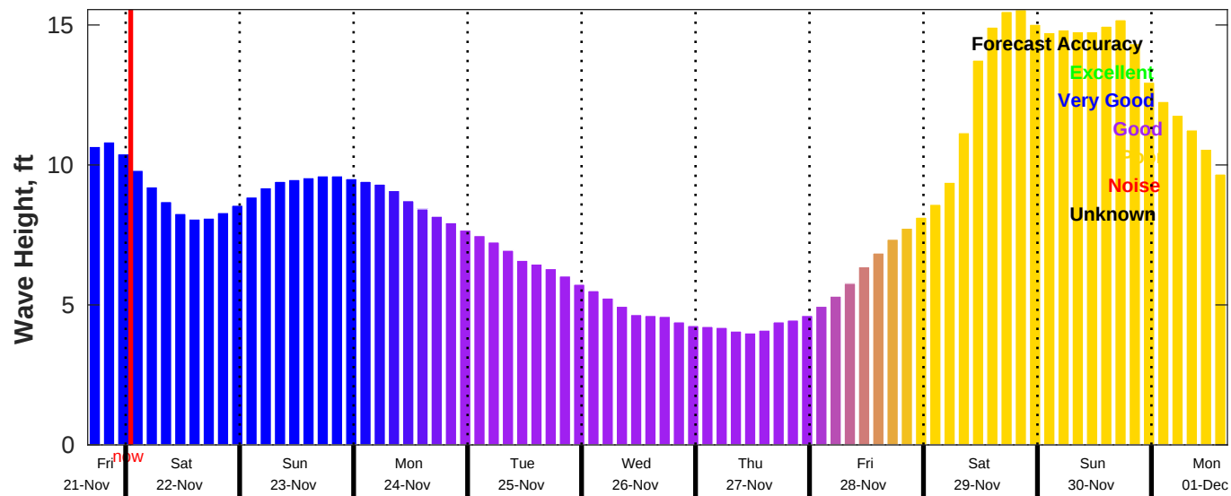
CMEMS Wave Forecast for NDBC 46011 from 21-Nov-2025 16:00:00 to 01-Dec-2025 16:00:00
