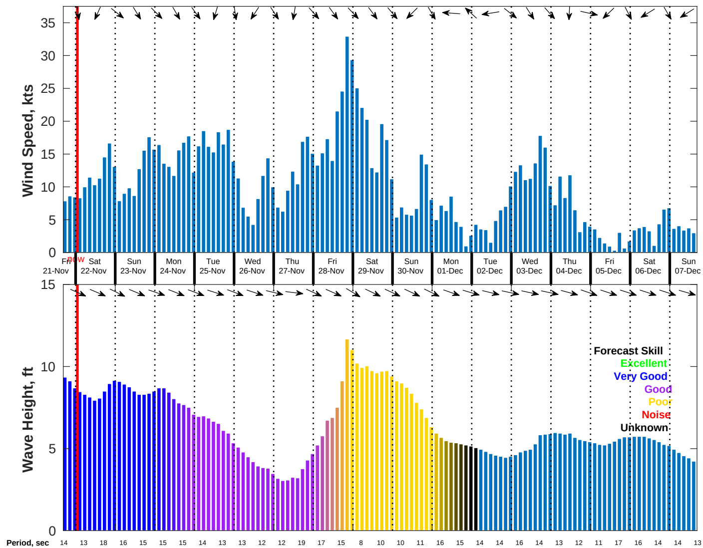
Wind & Wave Forecast for NDBC 46011 from 21-Nov-2025 16:00:00 to 07-Dec-2025 16:00:00
