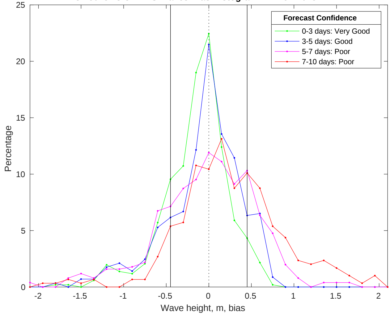
NDBC 46028 vs CMEMS Waves Bias Histogram: 22-Nov-2025
