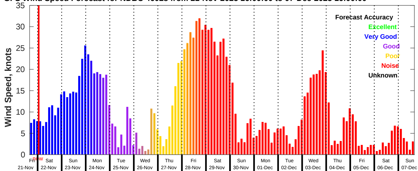
GFS Wind Speed Forecast for NDBC 46028 from 21-Nov-2025 16:00:00 to 07-Dec-2025 16:00:00
