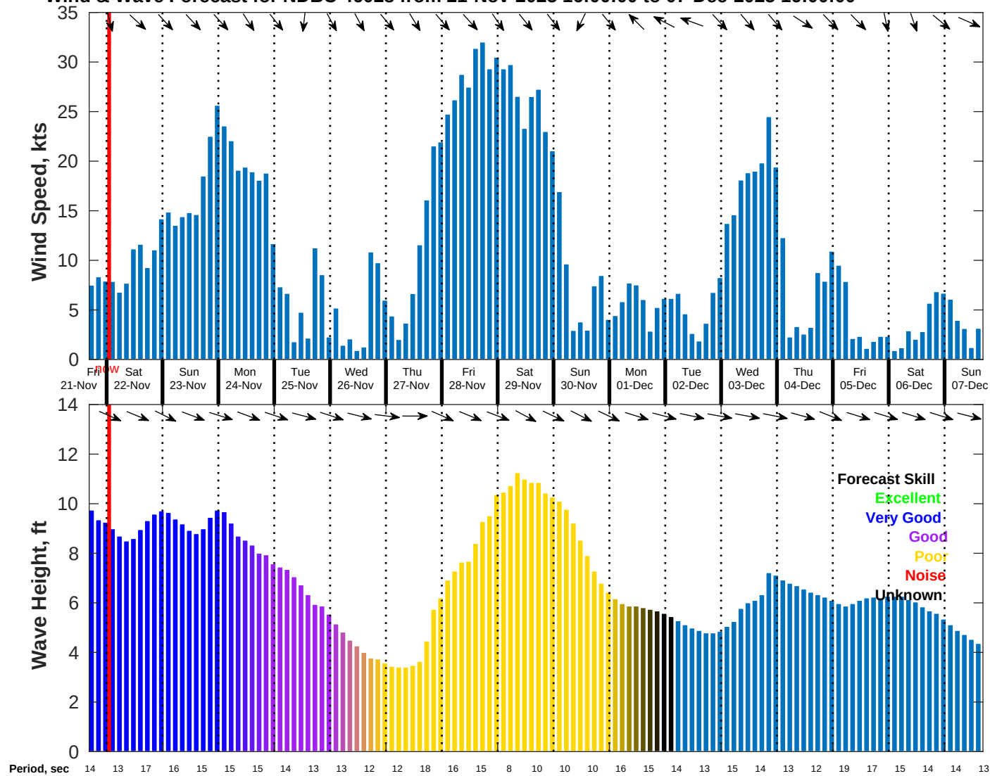
Wind & Wave Forecast for NDBC 46028 from 21-Nov-2025 16:00:00 to 07-Dec-2025 16:00:00
