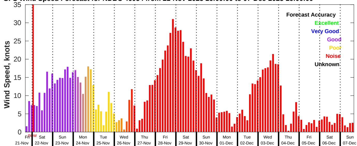
GFS Wind Speed Forecast for NDBC 46054 from 21-Nov-2025 16:00:00 to 07-Dec-2025 16:00:00
