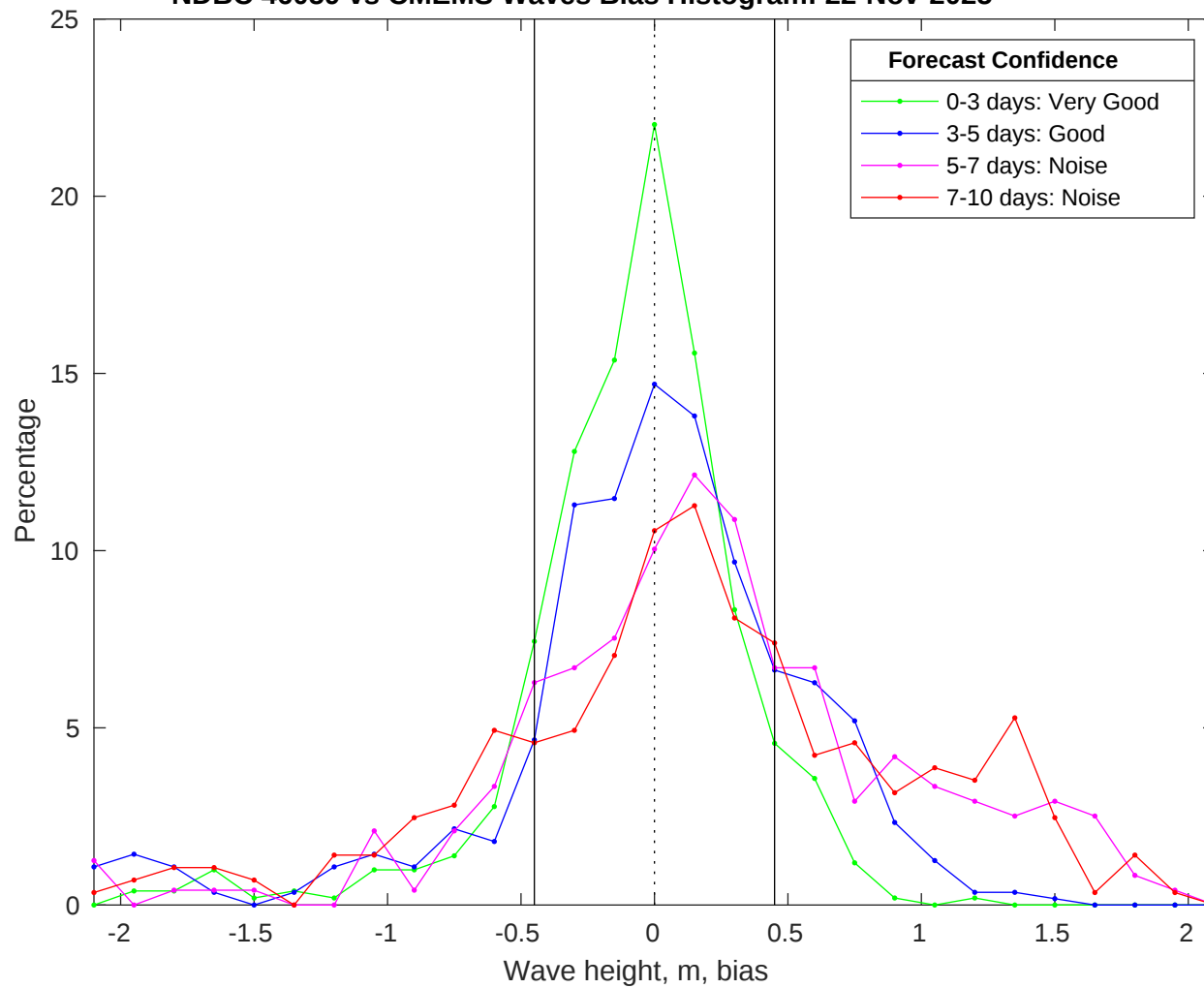
NDBC 46059 vs CMEMS Waves Bias Histogram: 22-Nov-2025
