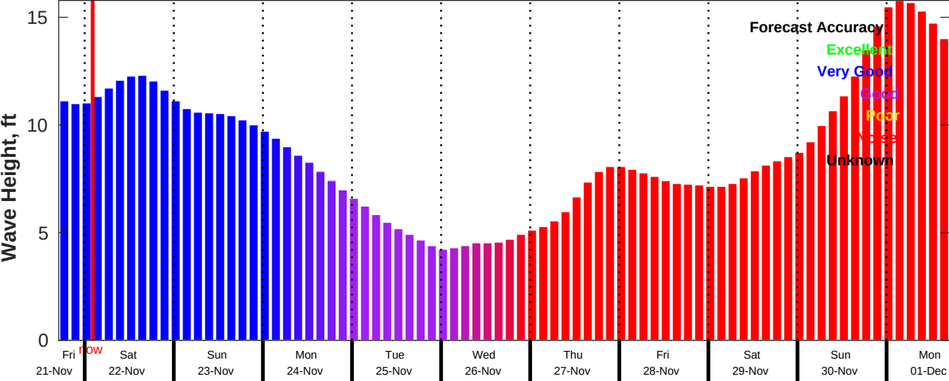
CMEMS Wave Forecast for NDBC 46059 from 21-Nov-2025 17:00:00 to 01-Dec-2025 17:00:00
