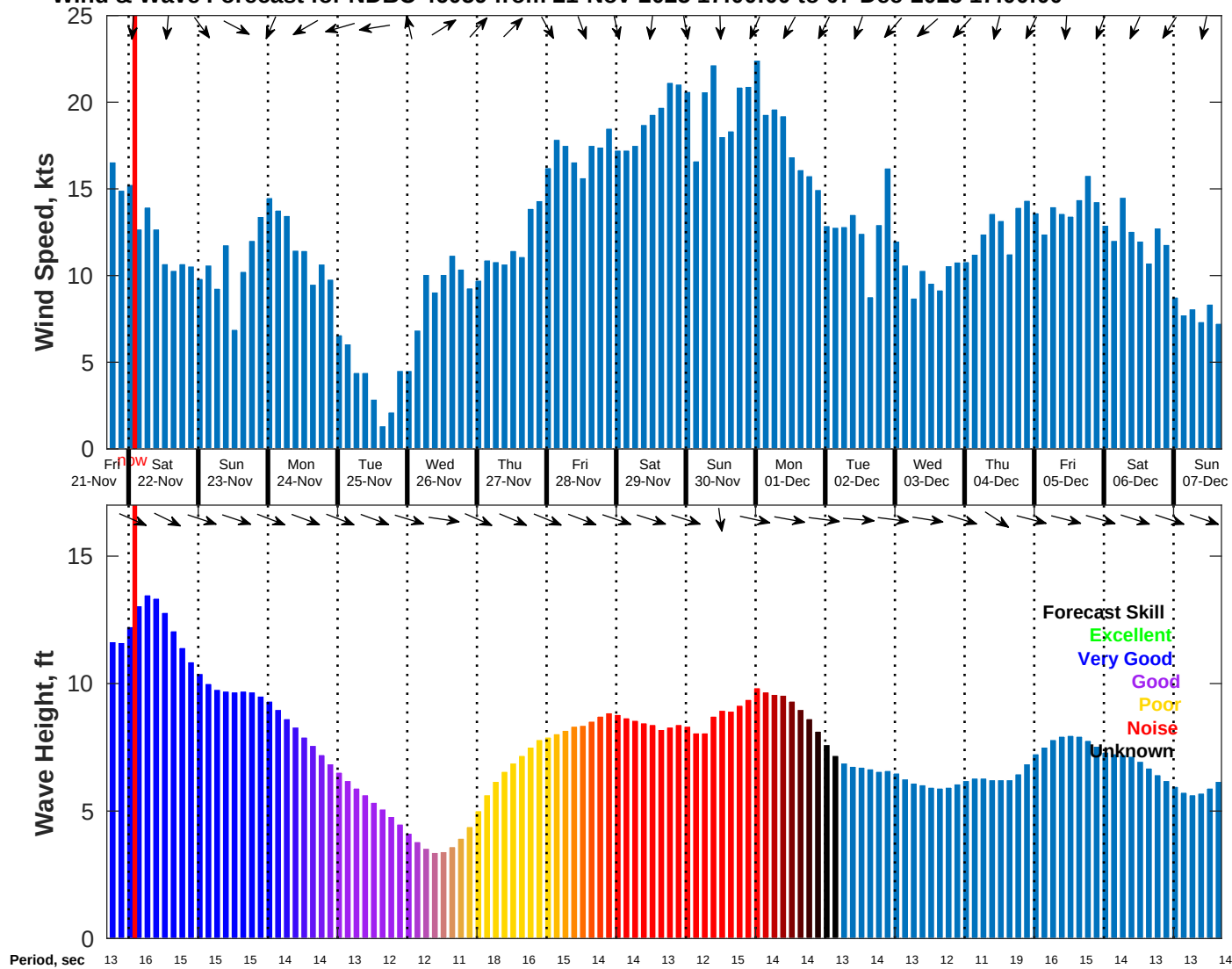
Wind & Wave Forecast for NDBC 46059 from 21-Nov-2025 17:00:00 to 07-Dec-2025 17:00:00
